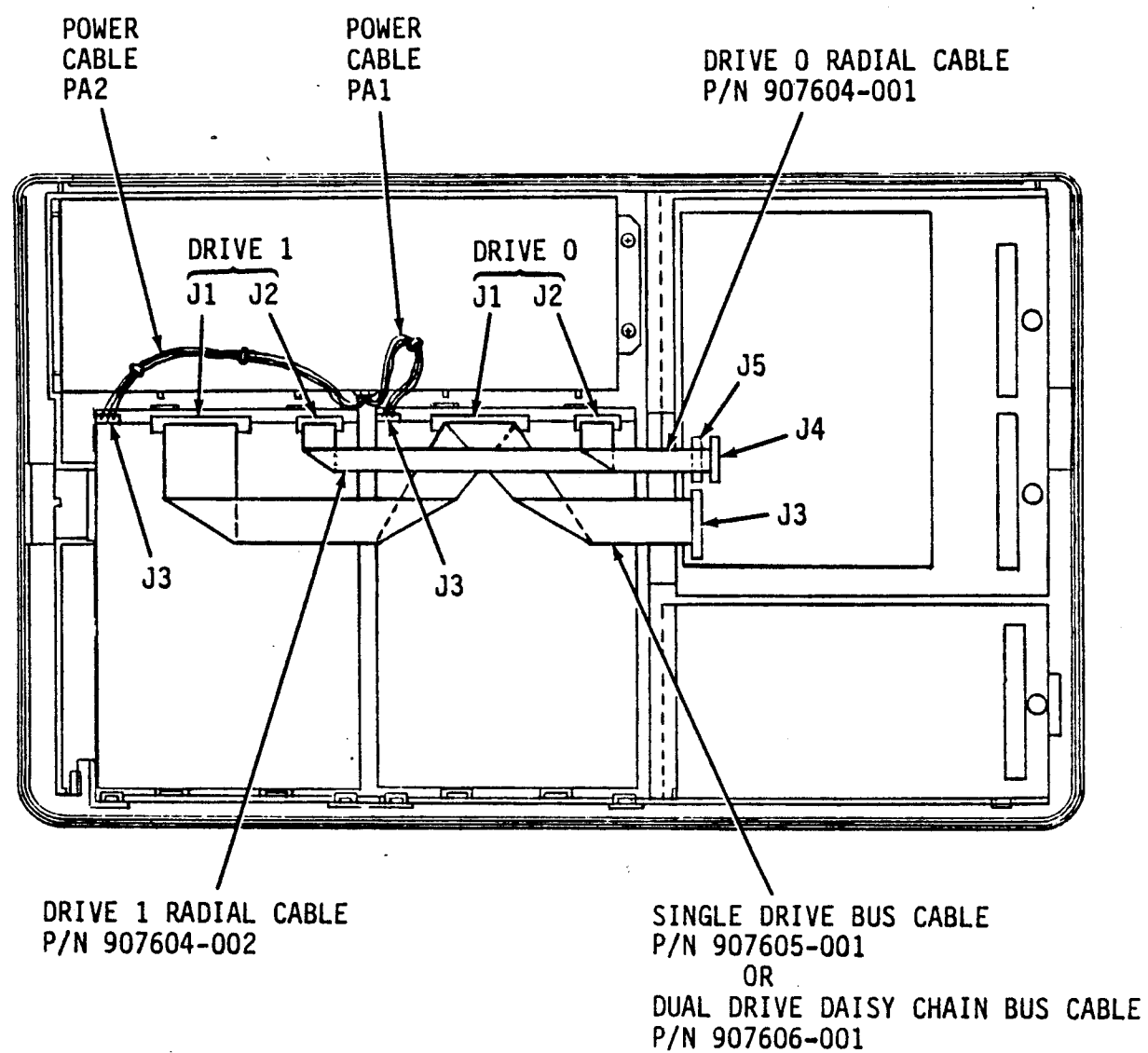
Figure 5-1. Disk Drive Removal/Replacement/Installation, Series 2000 Systems
