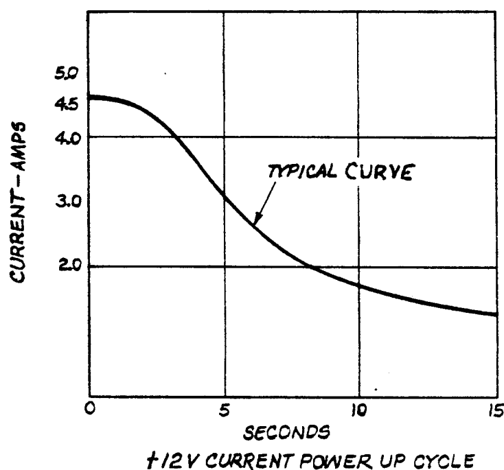
Figure 2-3. Motor Start Current Requirements
